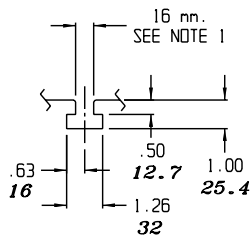
T-SLOT DETAIL
