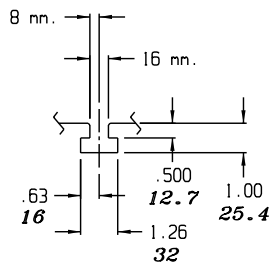
T-SLOT DETAIL
