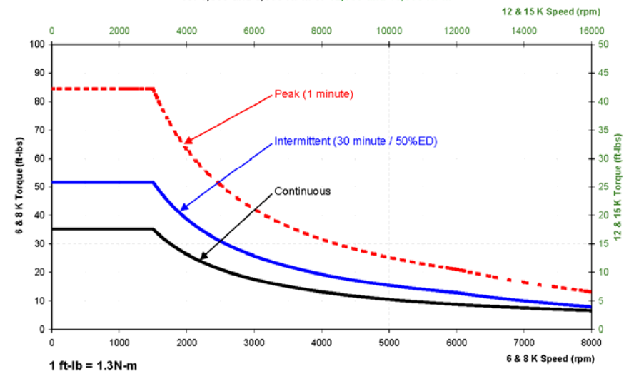
Torque Characteristics of 24/15 HP Single Winding Motor for 6,000 and 8,000 RPM or 12,000 and 15,000 RPM
